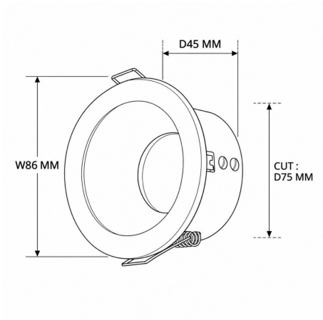
DIMENSION DRAWING
